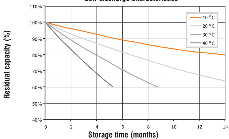
Self-discharge characteristics
